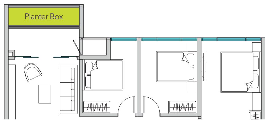
TYPE A1-A 1219 SQ.FT + 27 SQ.FT (Planter Box)
